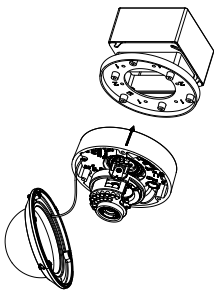
Figure 2-29 Secure Camera
