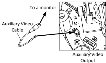
Figure 2-31 Connect Camera to a Monitor
